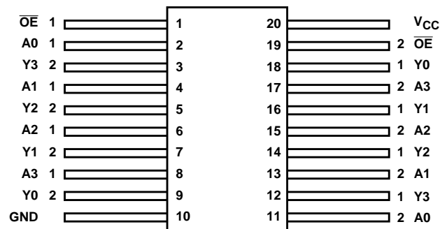
HCTS244KTR (FLATPACK), CDFF4-F20 TOP VIEW
